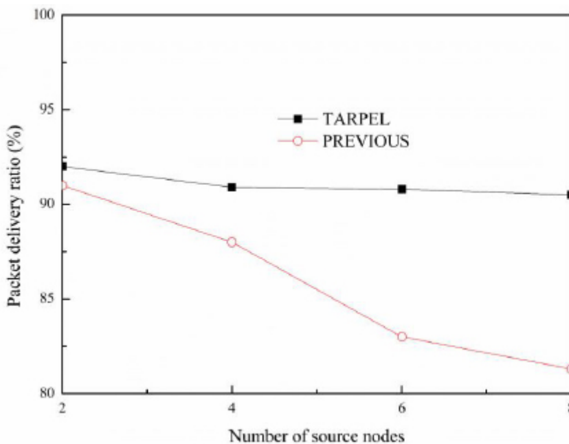
Fig. (1). Comparison of the packet delivery ratio.
